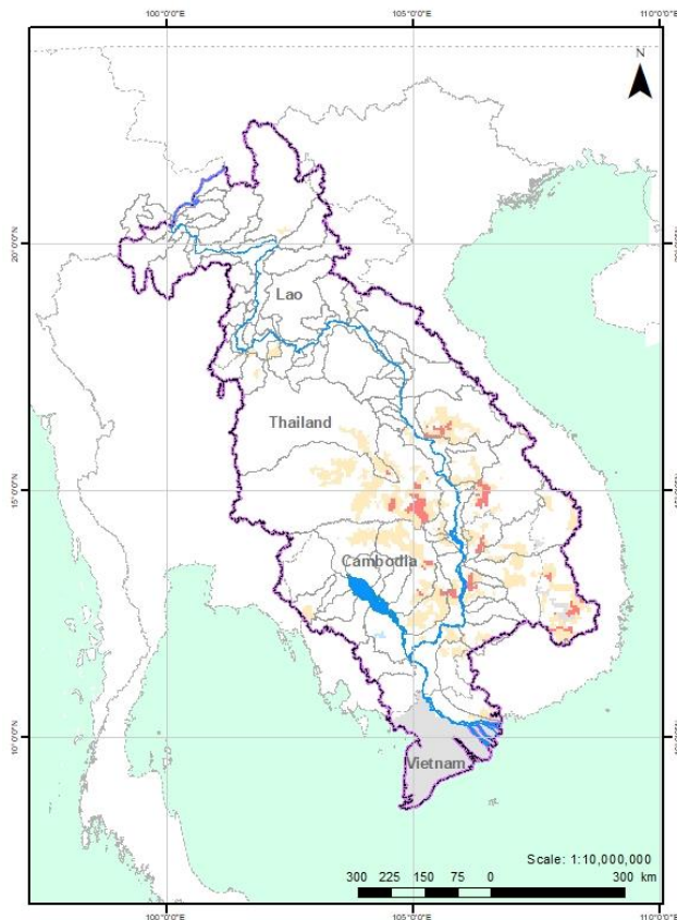
Figure 16. Index of Soil Water Fraction from 14 to 20 August 2023.
