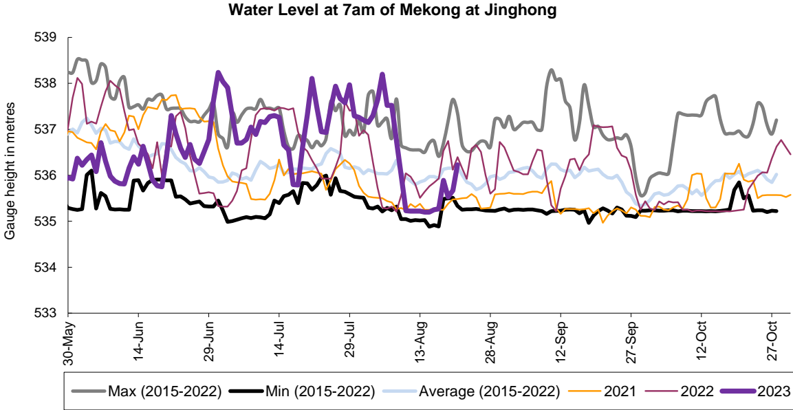
Figure 7. Water level at the Jinghong hydrological station up to 21 August 2023.
