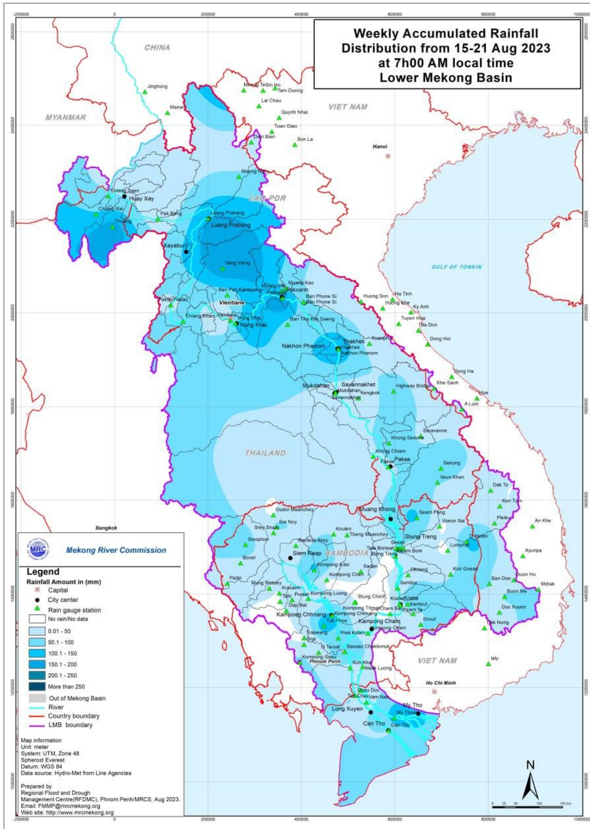
Figure 5. Weekly rainfall distribution over the LMB during 15-21 August 2023.
