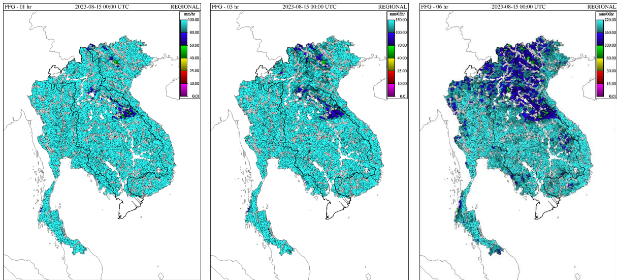
Figure 14. Flash Flood Guidance for the next 1-hr, 3-hr and 6-hr on August 15
