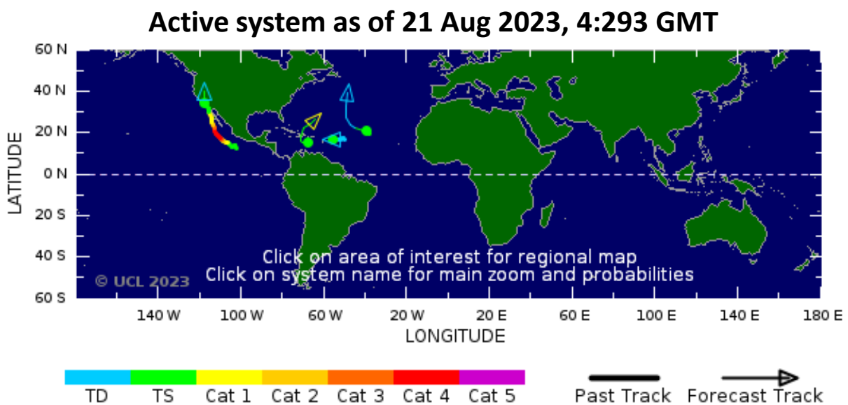
Figure 3. A tropical depression risk observed on 21 August 2023.
