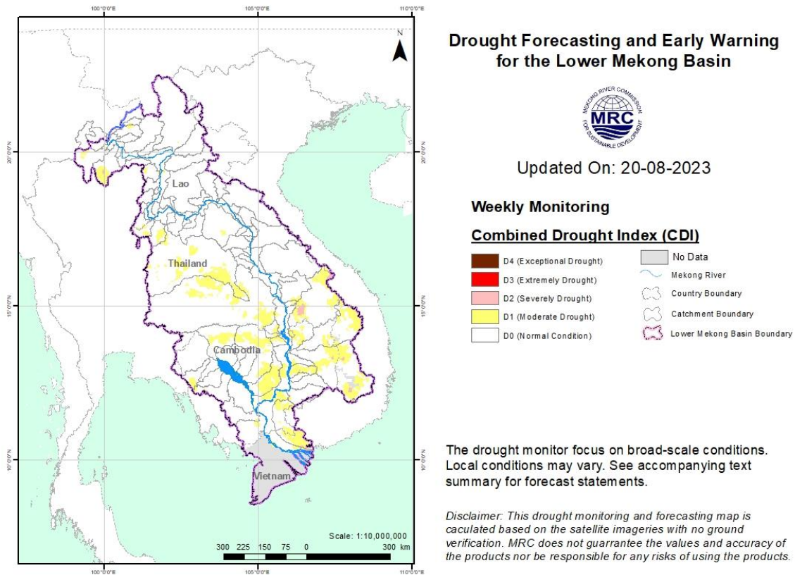
Figure 17. Weekly Combined Drought Index from 14 to 20 August 2023.
