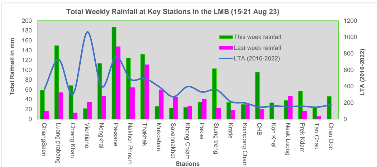
Figure 4. Weekly total rainfall at key stations in the LMB during 15-21 August 2023.
