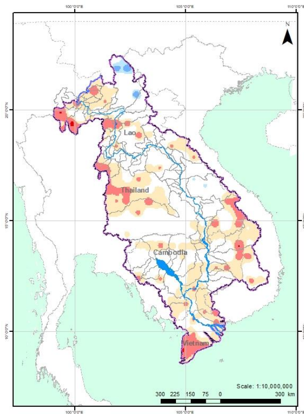
Figure 15. Weekly standardized precipitation index from 14 to 20 August 2023.
